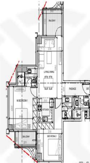
APARTMENT - 2 BED ROOM - TYPE 2B-B
